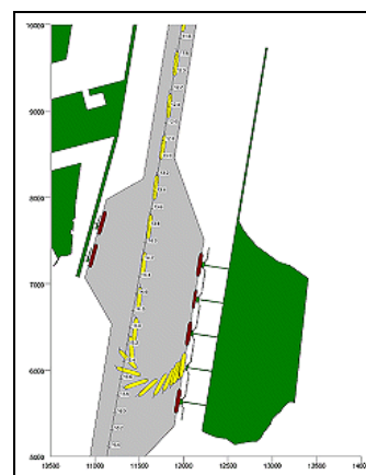
Figure 5: Track plot of simulation
